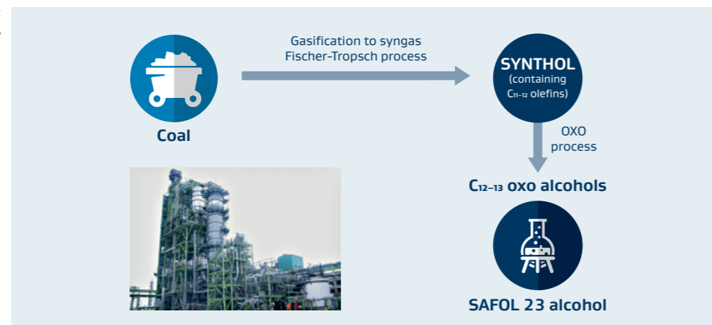
Figure 1: Coal-to-alcohol process
